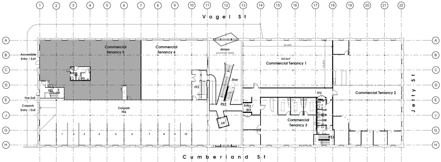
Overall Existing First Floor Plan 1:200
